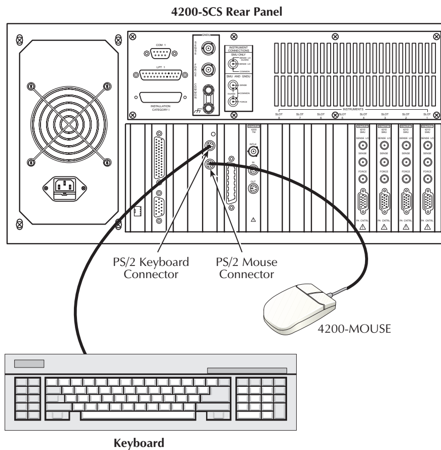
Figure 1 Connections
