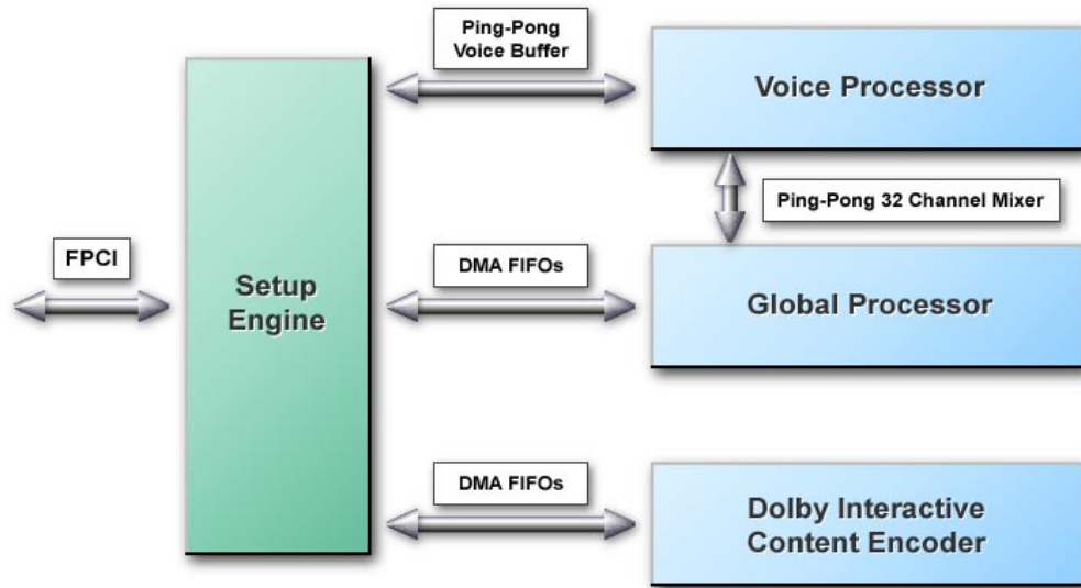
Figure 8. A high-level block diagram of the APU
